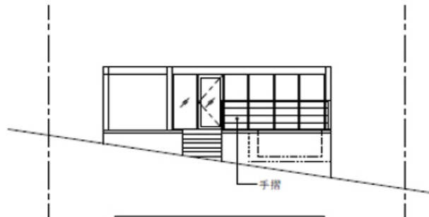
FACADE EAST 1/150
